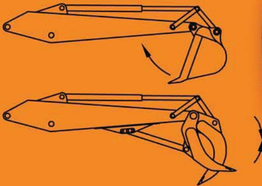
Bucket Curl = GPG Close
